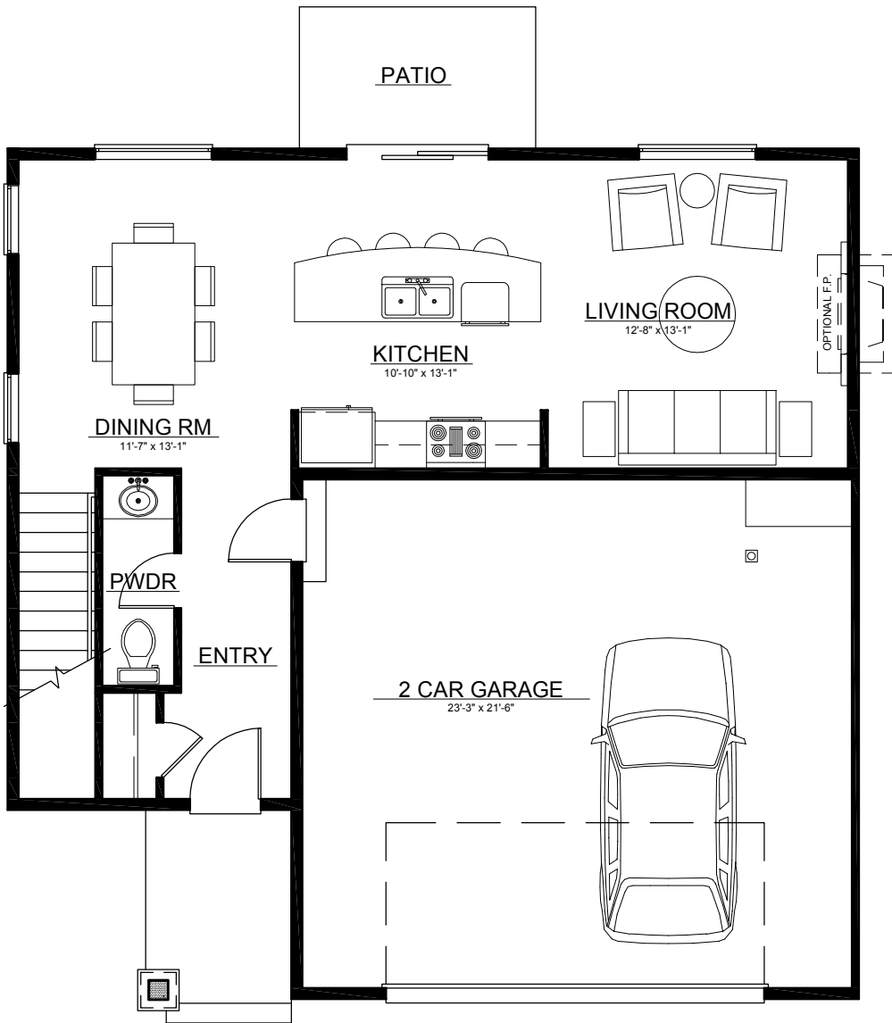
FIRST FLOOR
